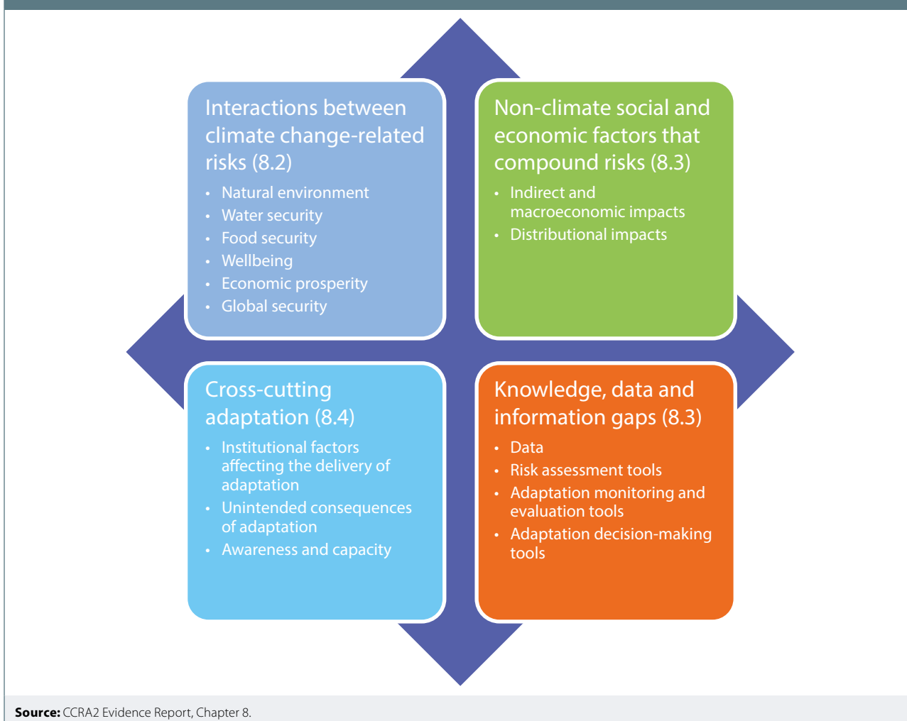
Figure SR.A6: Cross-cutting issues affecting climate change risks
