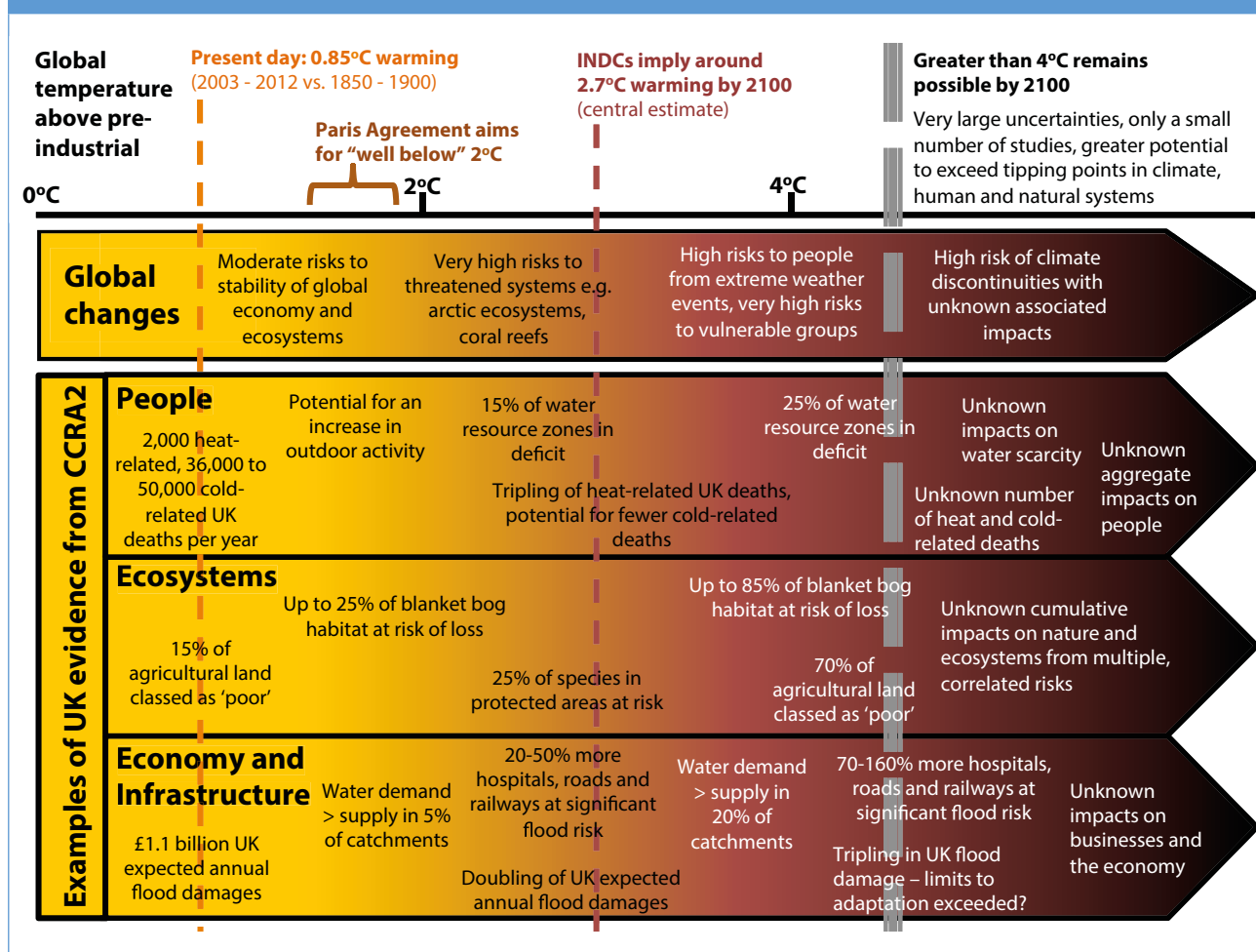
Figure SR.7: Magnitude of UK climate change impacts for various degrees of global warming
