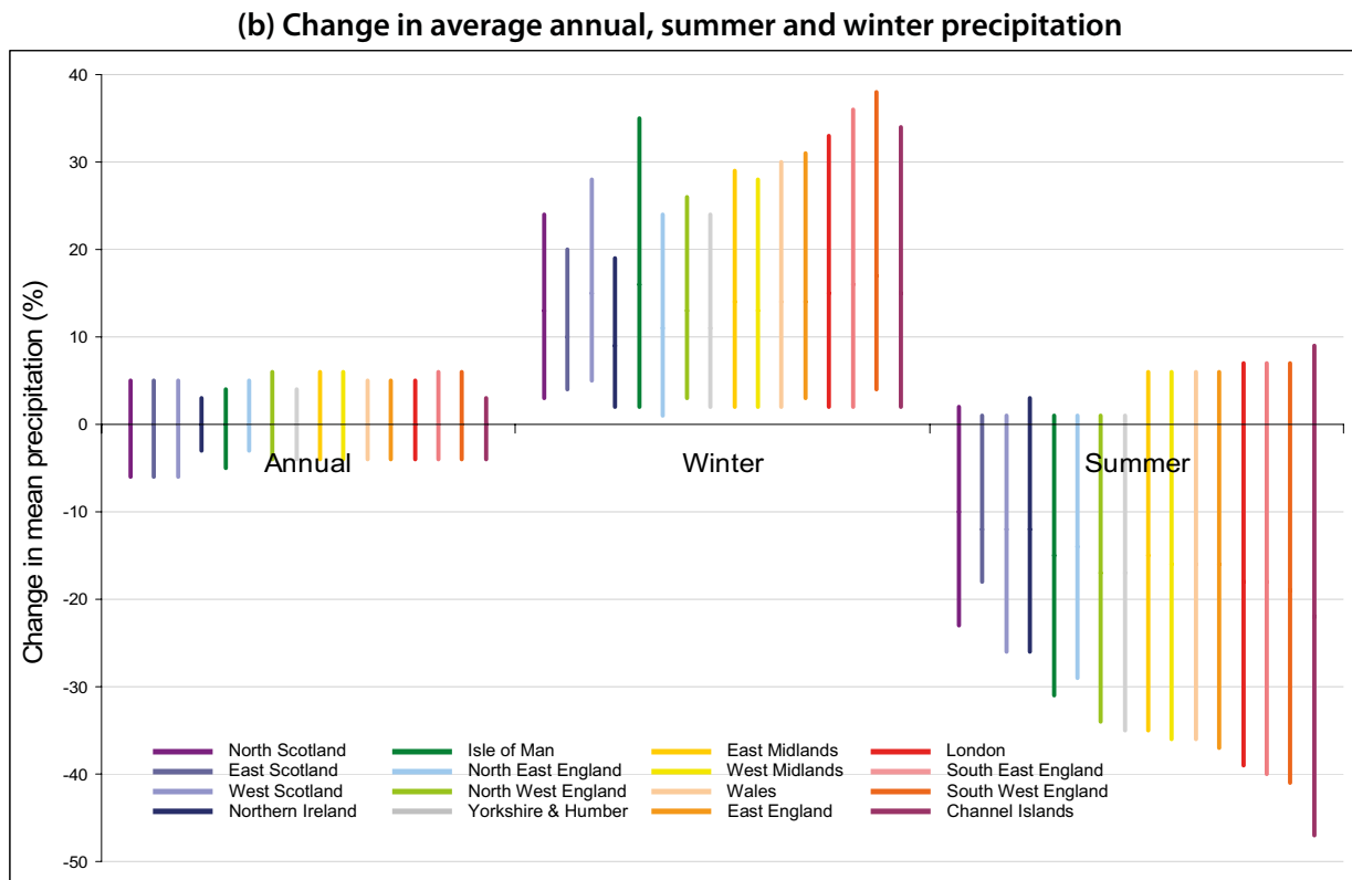
Figure SR.6: UKCP09 projections for temperature and rainfall
